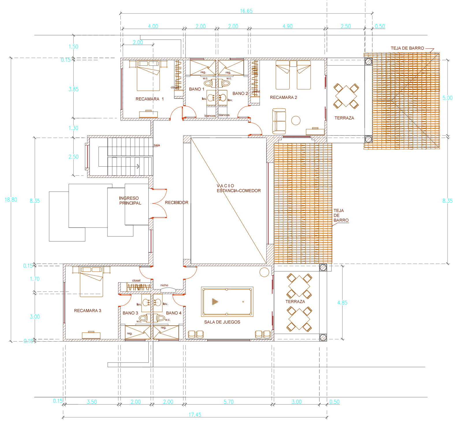
VILLA "D" PLANTA ALTA (upper level)
